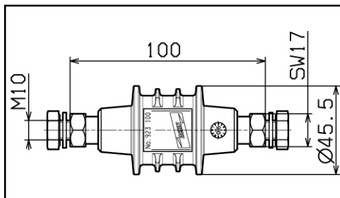
Dimension drawing EXFS 100
